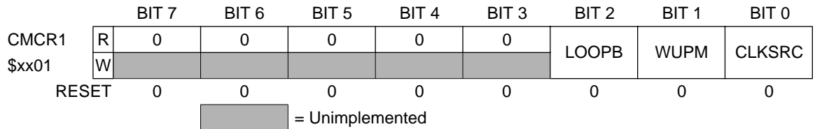
Figure 16. Module control register 1 (CMCR1)
