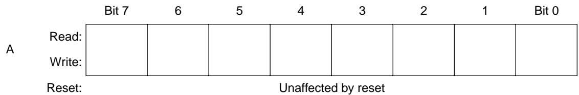
Figure 1. Accumulator (A)
