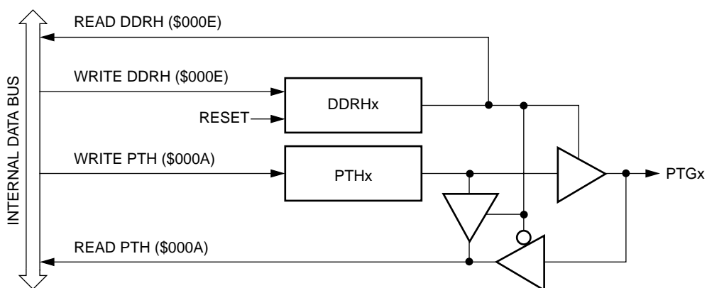
Figure 24. Port H I/O circuit
