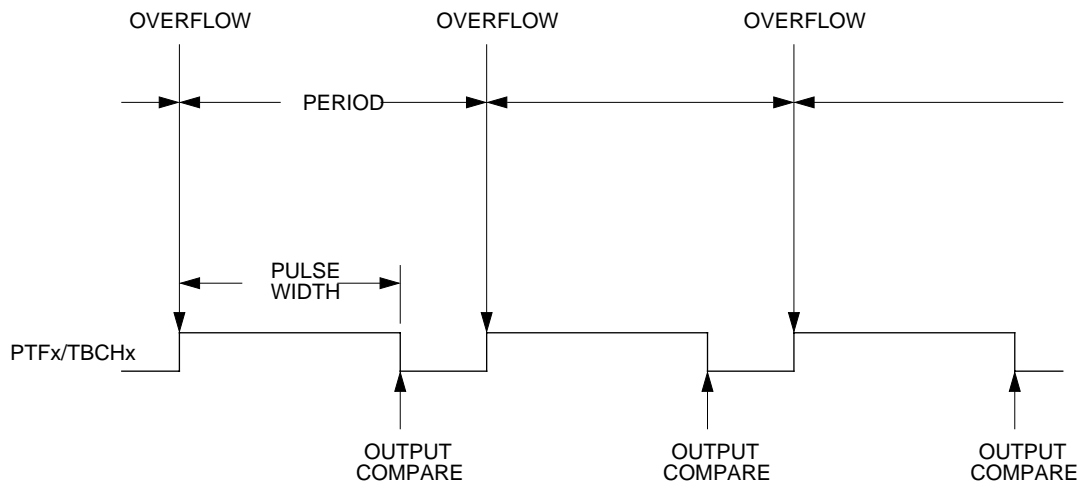
Figure 2. PWM period and pulse width
