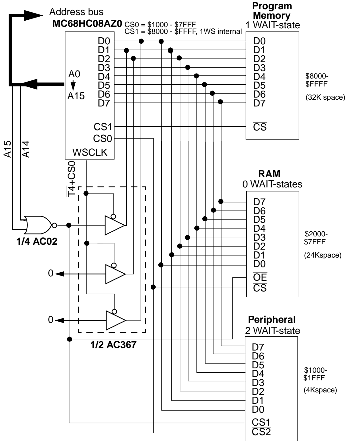
Figure 7. Simple address space decode with different WAIT states
