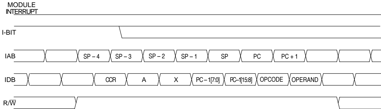
Figure 9. Interrupt recovery
