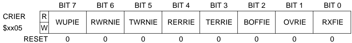
Figure 20. Receiver Interrupt Enable Register
