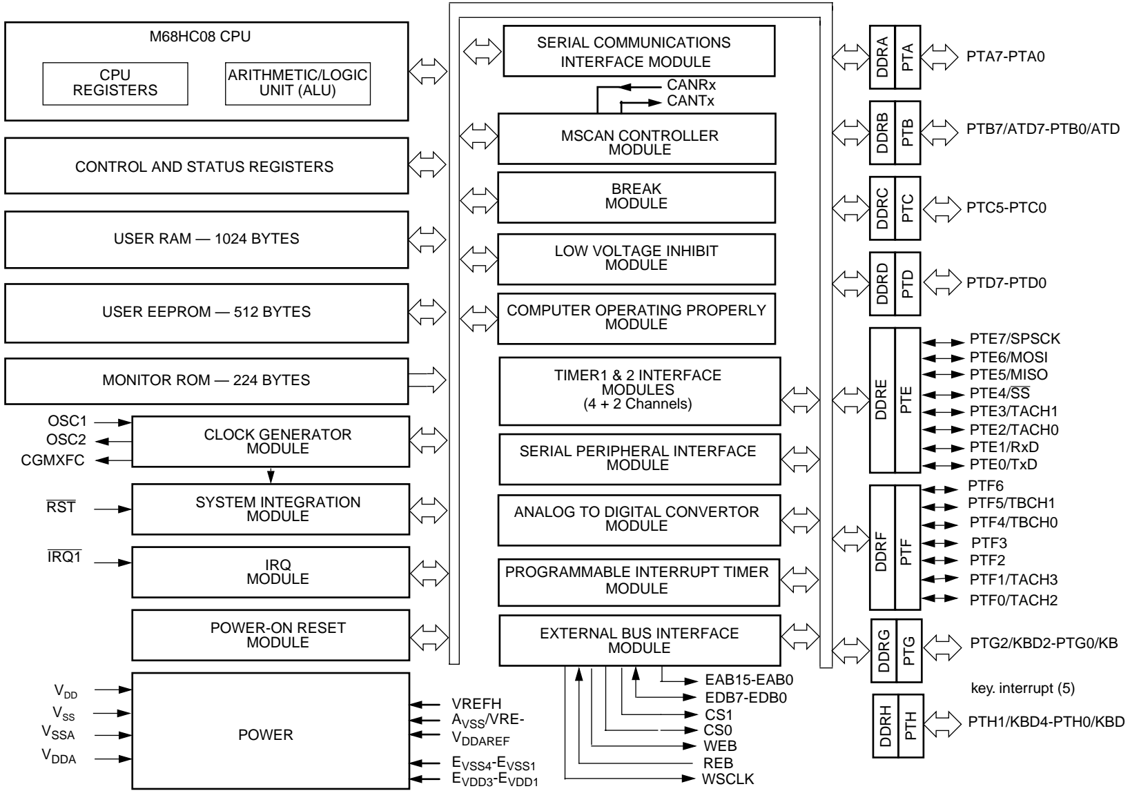
Figure 1. MC68HC08AZ0 MCU block diagram
