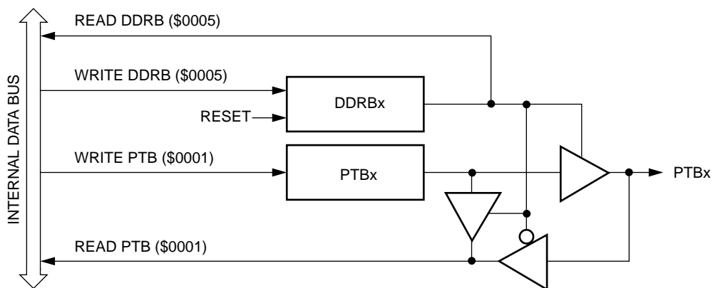
Figure 6. Port B I/O circuit
