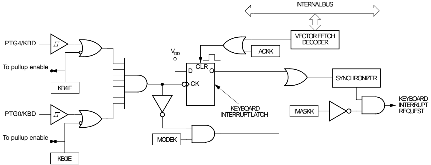
Figure 5. Keyboard module block diagram
