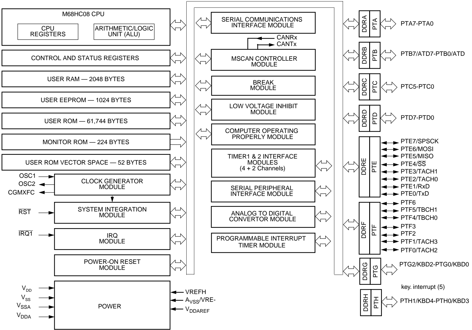
Figure 17. MC68HC08AZ60 MCU block diagram
