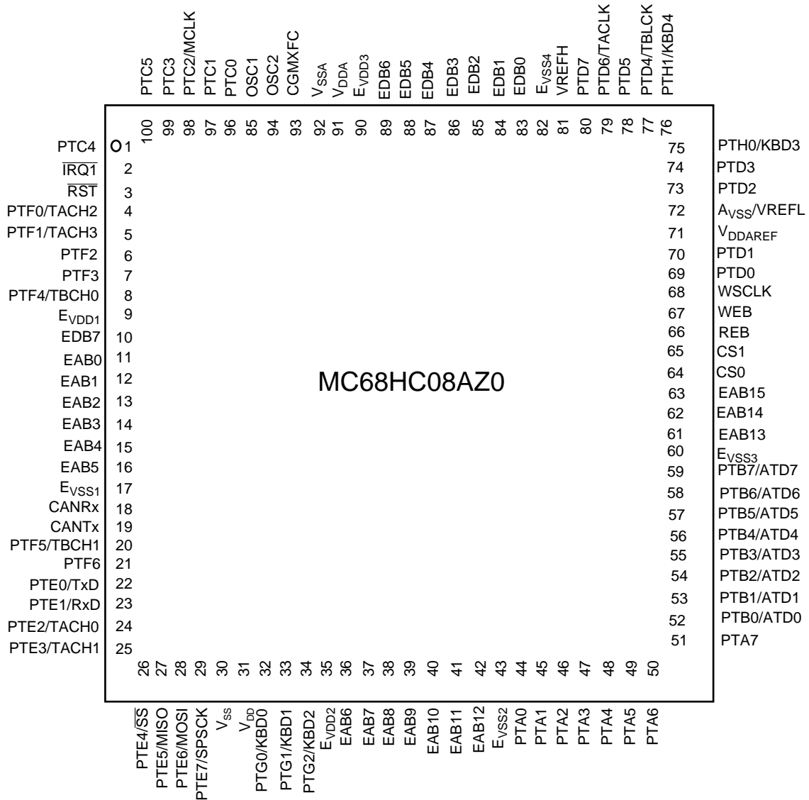
Figure 2. MC68HC08AZ0 100TQFP pin assignments
