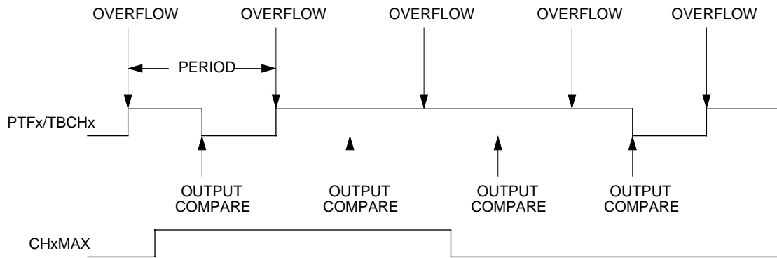
Figure 7. CHxMAX latency
