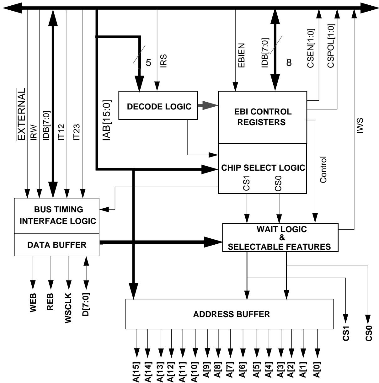
Figure 4. EBI block diagram
