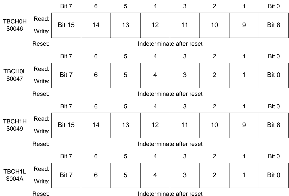
Figure 8. TIMB channel registers (TBCH0H/L–TBCH1H/L)
