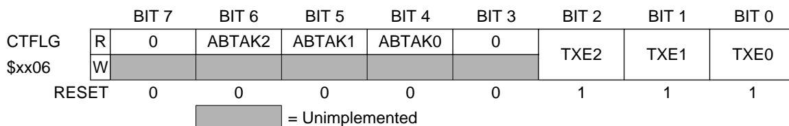
Figure 21. Transmitter Flag Register
