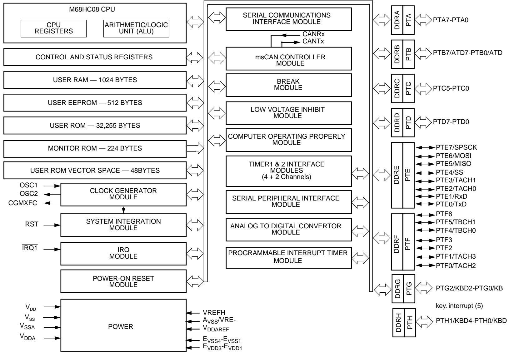
Figure 1. MC68HC08AZ32 MCU block diagram
