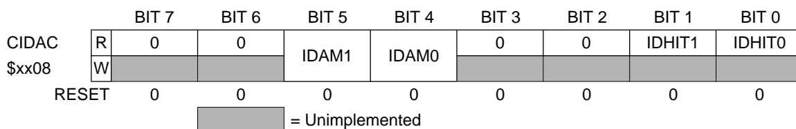
Figure 22. Identifier Acceptance Control Register
