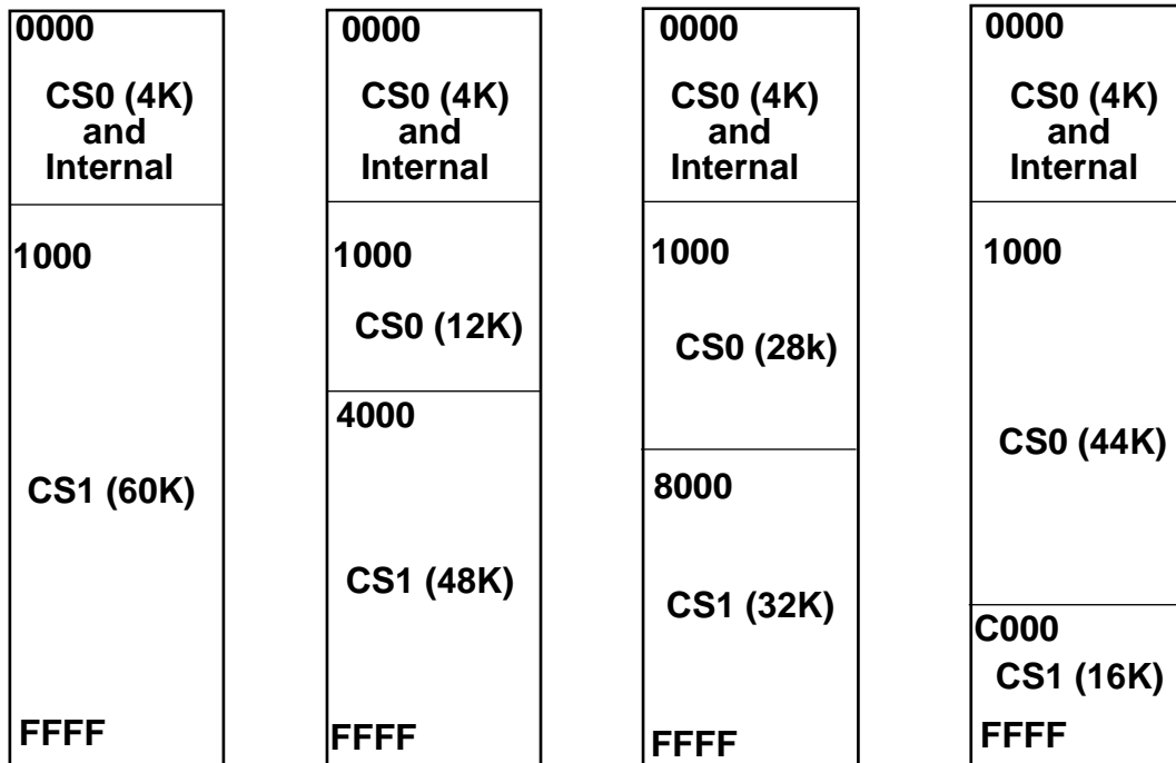
Figure 5. Software controlled chip-select combinations
