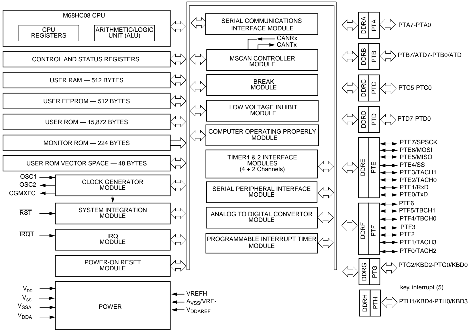
Figure 11. MC68HC08AZ16 MCU block diagram
