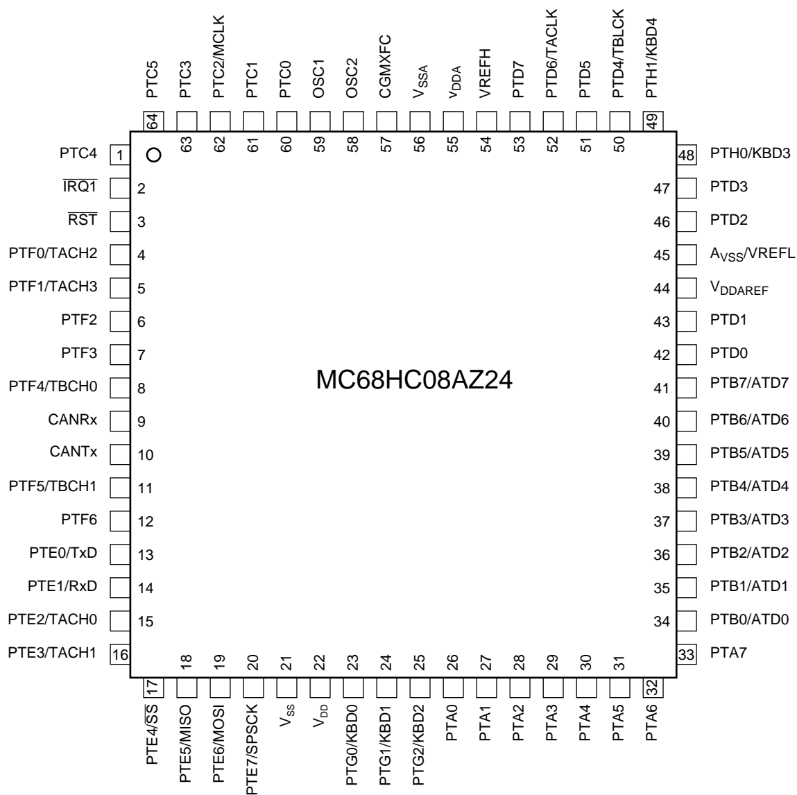
Figure 15. MC68HC08AZ24 64 QFP pin assignments
