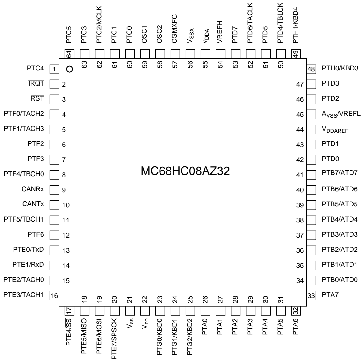
Figure 2. 64 QFP pin assignments
