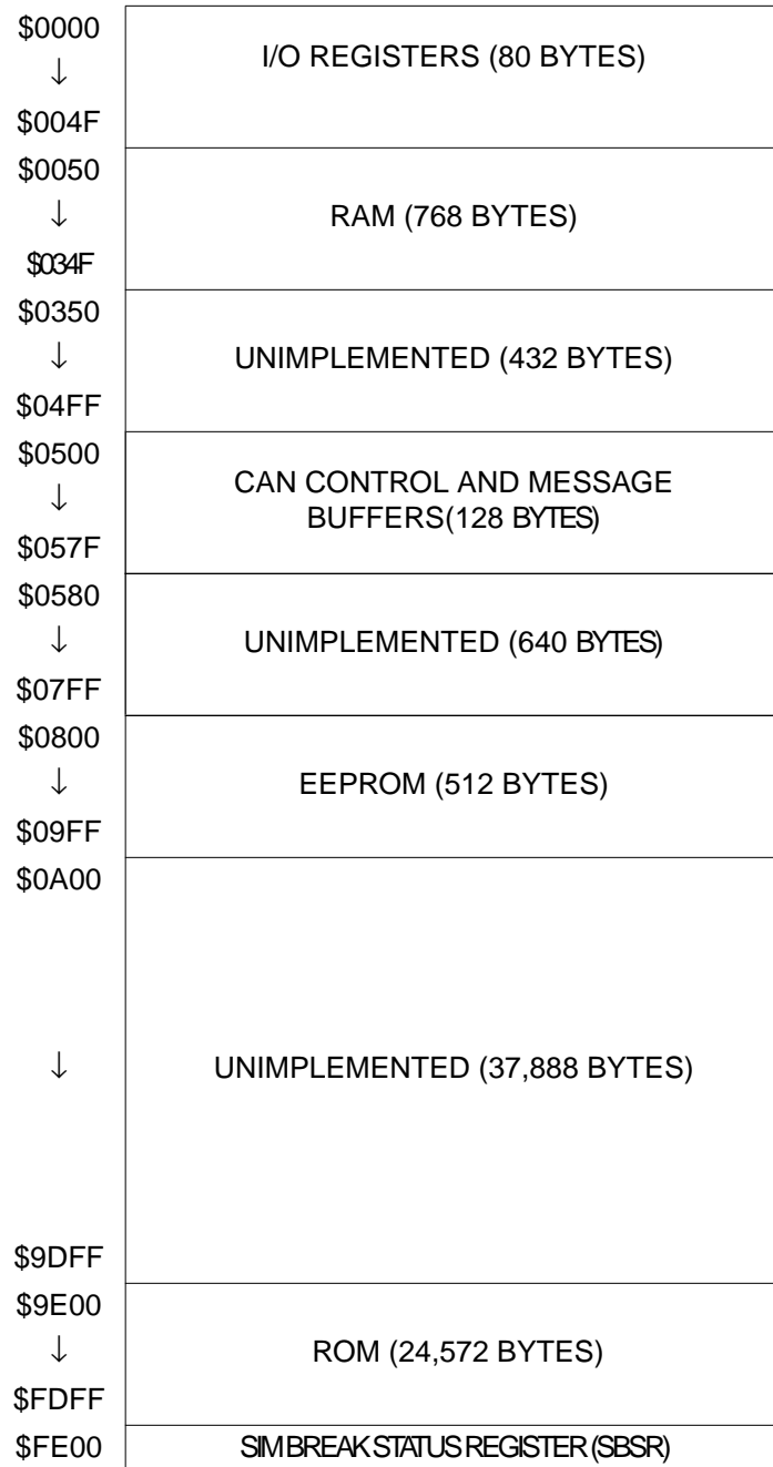
Figure 16. MC68HC08AZ24 Memory map
