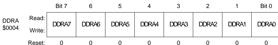
Figure 2 Data direction register A (DDRA)
