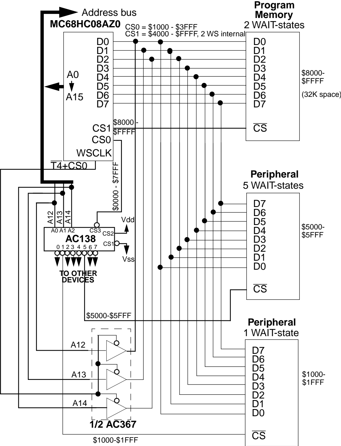
Figure 8. WAIT state selection for multiple I/O peripherals
