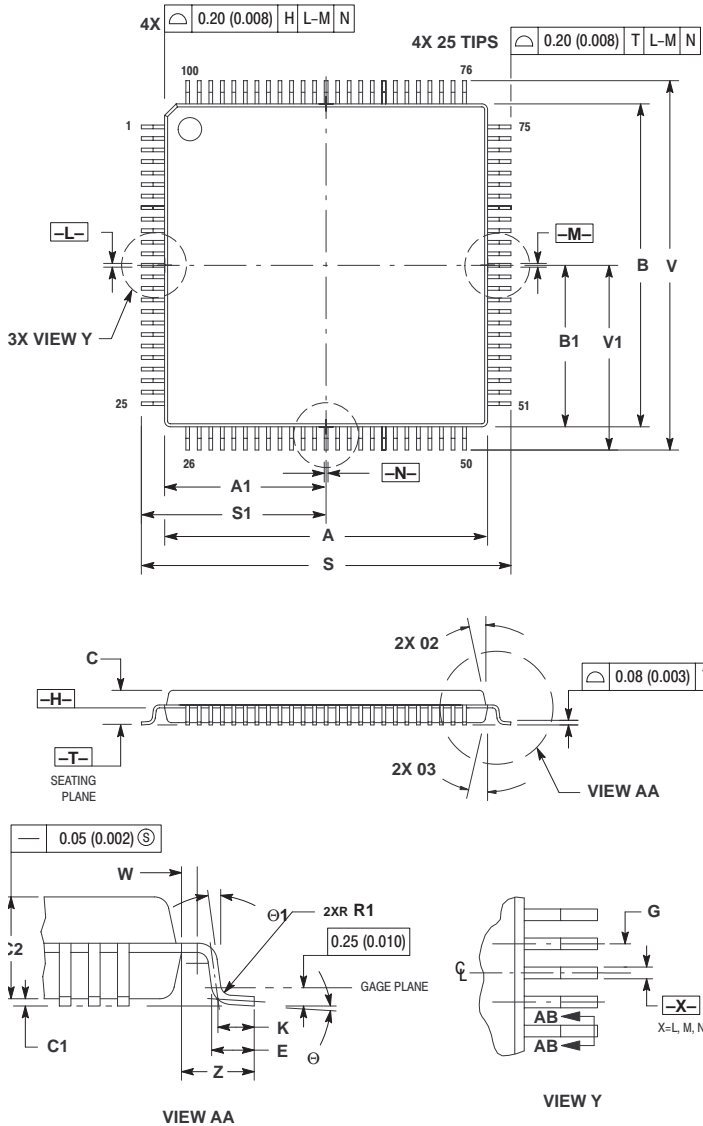
Figure 6. 100-pin TQFP (case #983)
