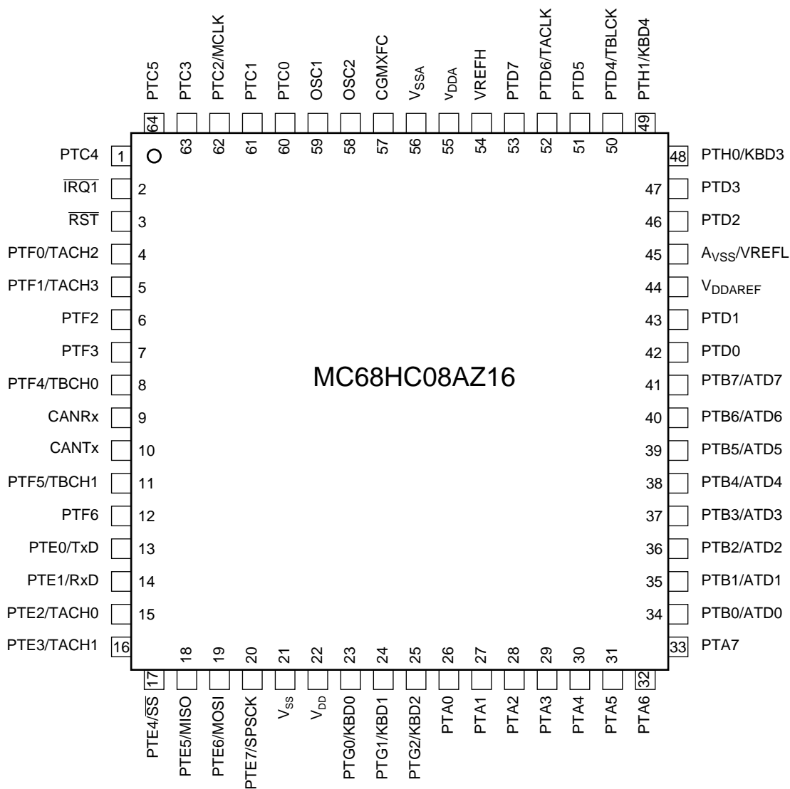
Figure 12. MC68HC08AZ16 64 QFP pin assignments
