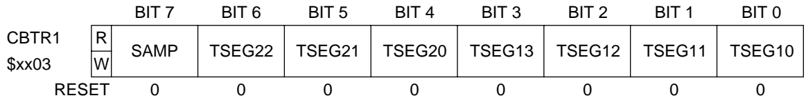
Figure 18. Bus timing register 1
