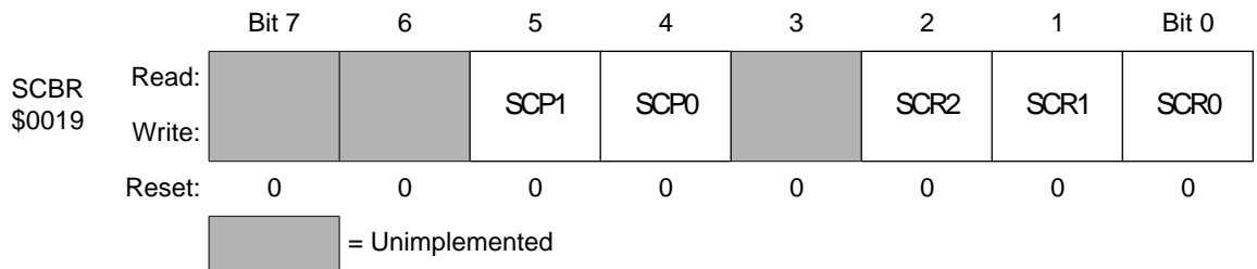
Figure 12. SCI Baud Rate Register (SCBR)
