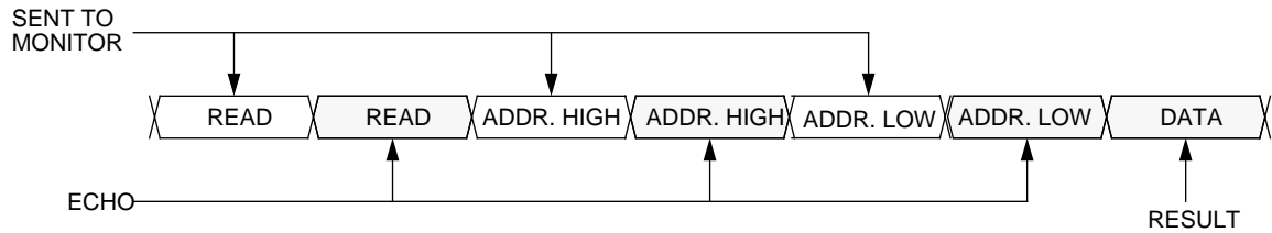
Figure 4. Read transaction
