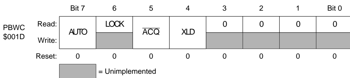
Figure 7. PLL bandwidth control register (PBWC)
