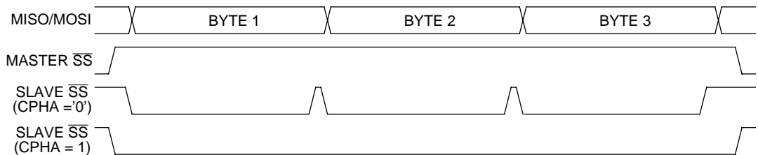
Figure 5. CPHA/ \overline{SS} timing
