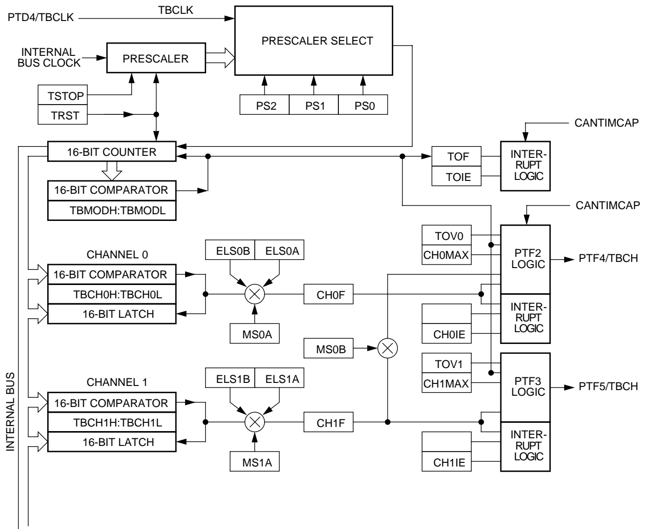
Figure 1. TIMB block diagram
