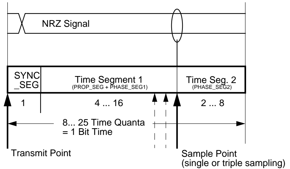
Figure 8. Segments within the bit time
