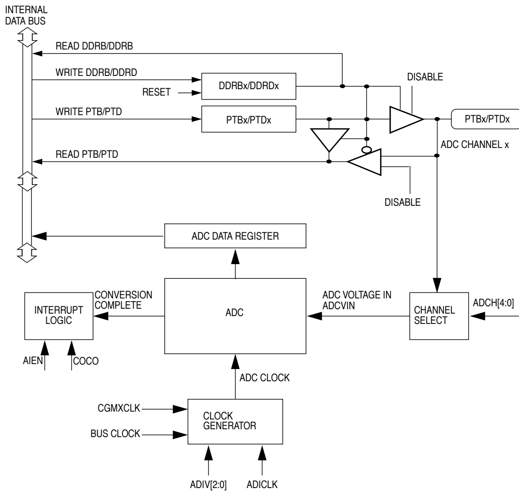
Figure 1. ADC-15 Block Diagram
