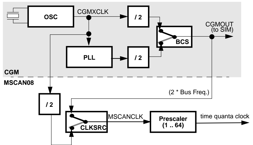
Figure 7. Clocking scheme
