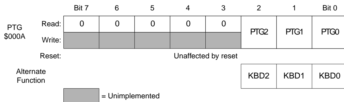
Figure 19. Port G data register (PTG)
