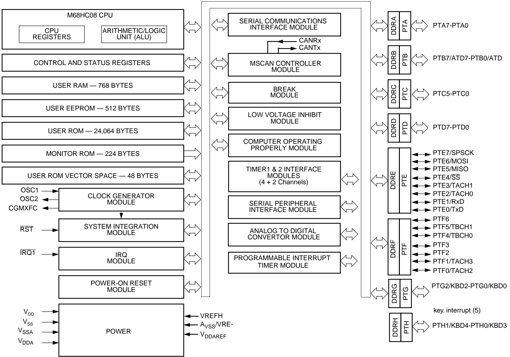
Figure 14. MC68HC08AZ24 MCU block diagram
