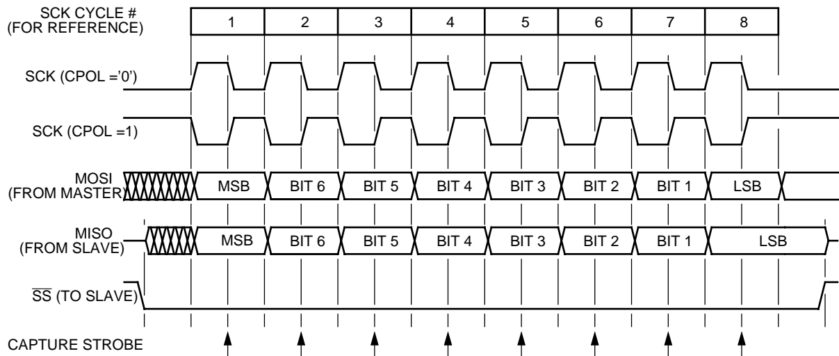
Figure 6. Transmission format (CPHA = '1')
