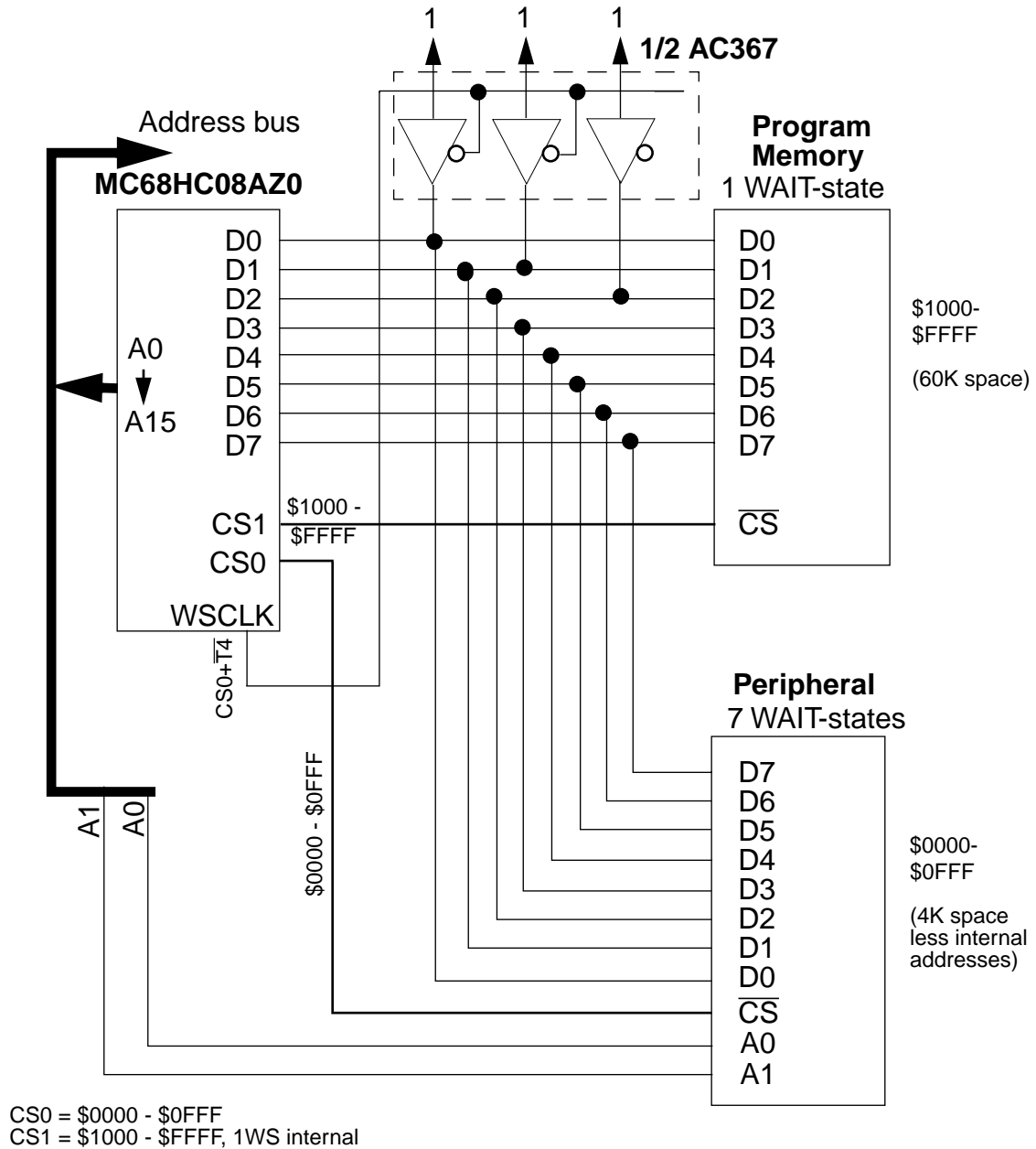
Figure 6. Defining WAIT states for EXIT addresses below $1000
