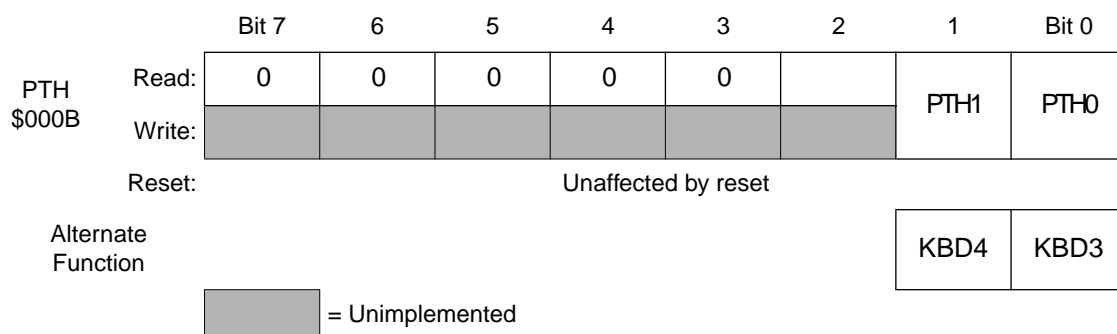
Figure 22. Port H data register (PTH)
