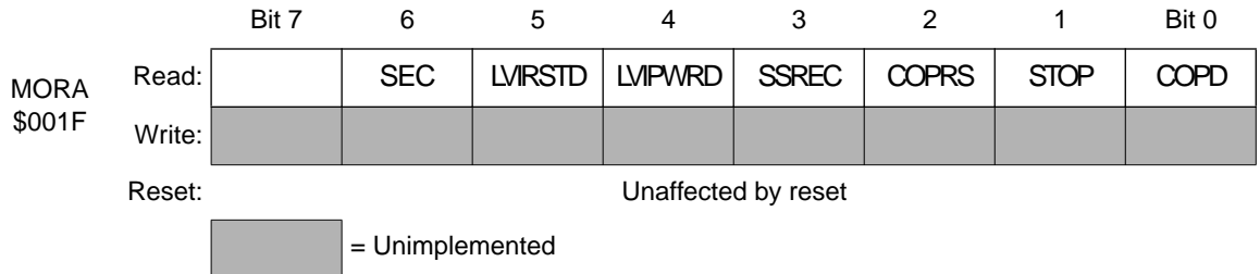
Figure 9. Mask option register A (MORA)
