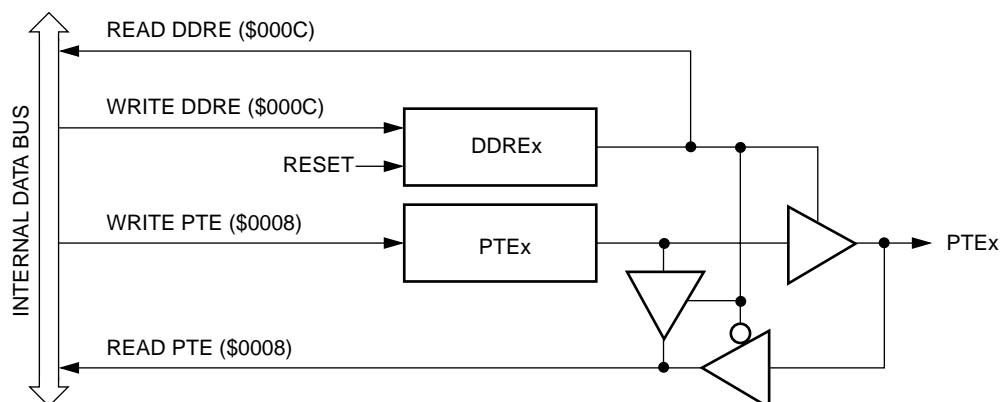
Figure 15. Port E I/O circuit
